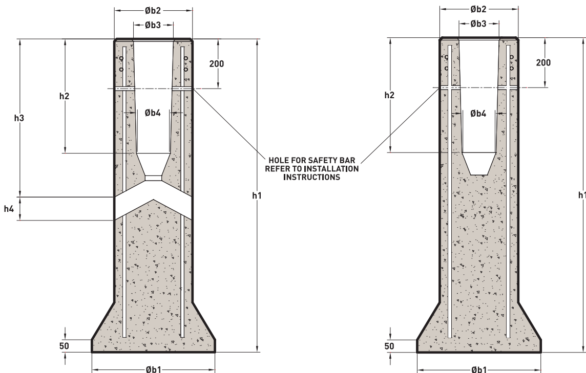
WITH CABLE DUCT FOR ILLUMINATED SIGNS AND LIGHTING COLUMNS
